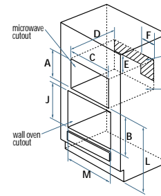
wall oven + microwave installation
