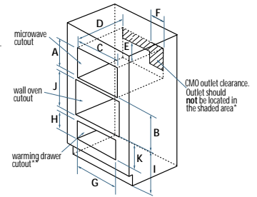
wall oven + microwave + warming drawer installation
