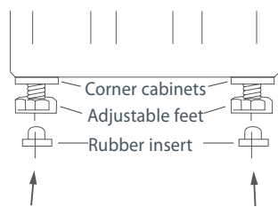
Fig.7 Adjusting leveling feet
