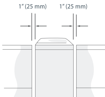
Fig.8 Minimum clearance
