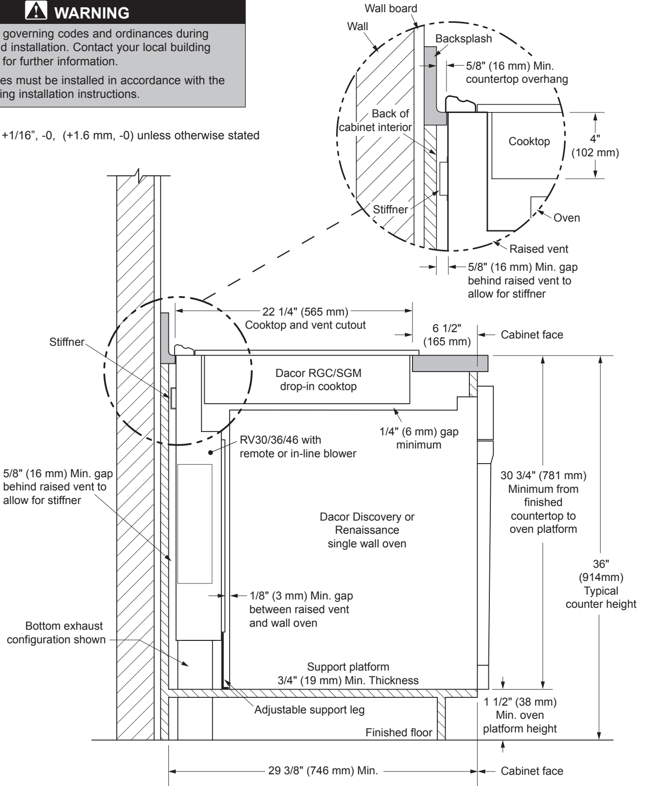
Cutaway Side View
