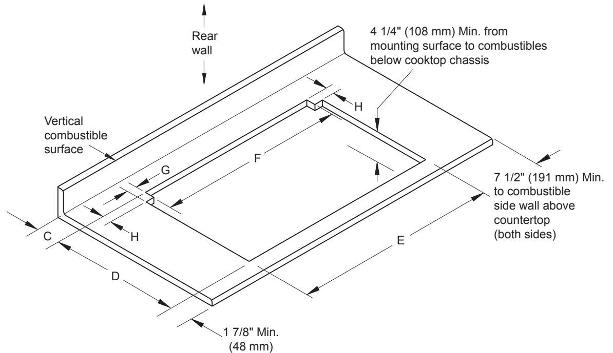
Figure 2 - Notched Countertop Cutout Diagram (SGM466 only)
