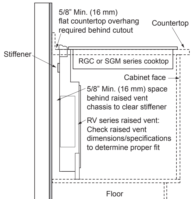
Side View - RGC/SGM Series Cooktop with RV Series Raised Vent
