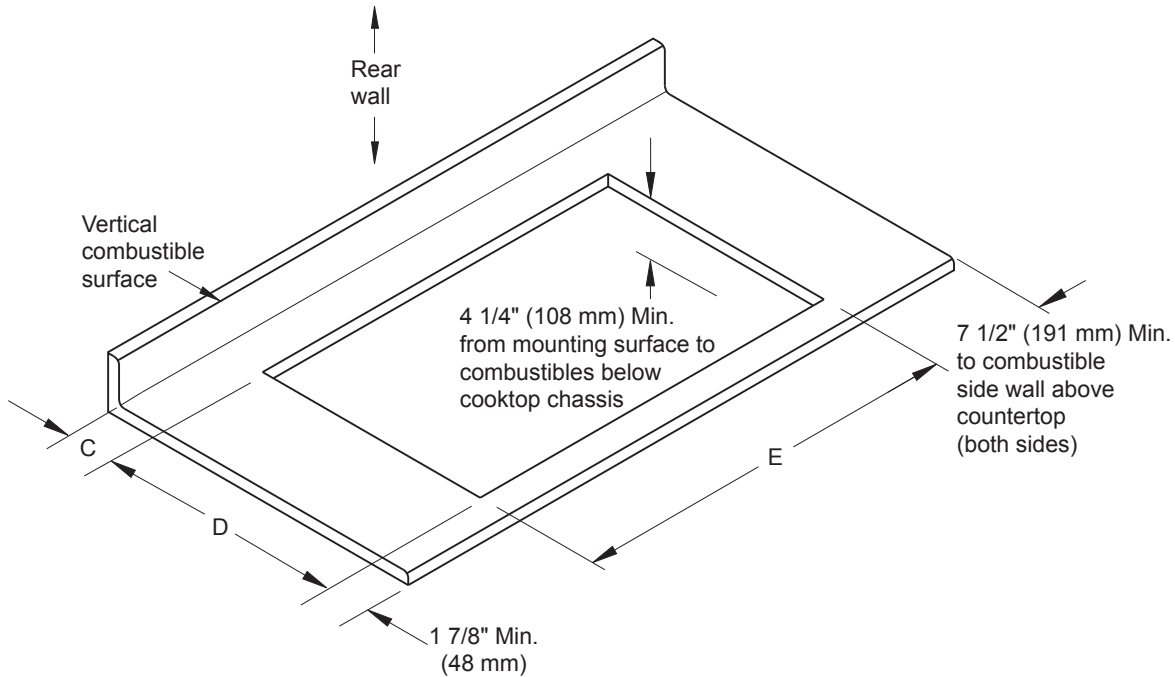
Figure 1 - Square Countertop Cutout Diagram
