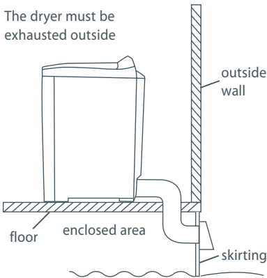
Fig.8 Exterior venting
