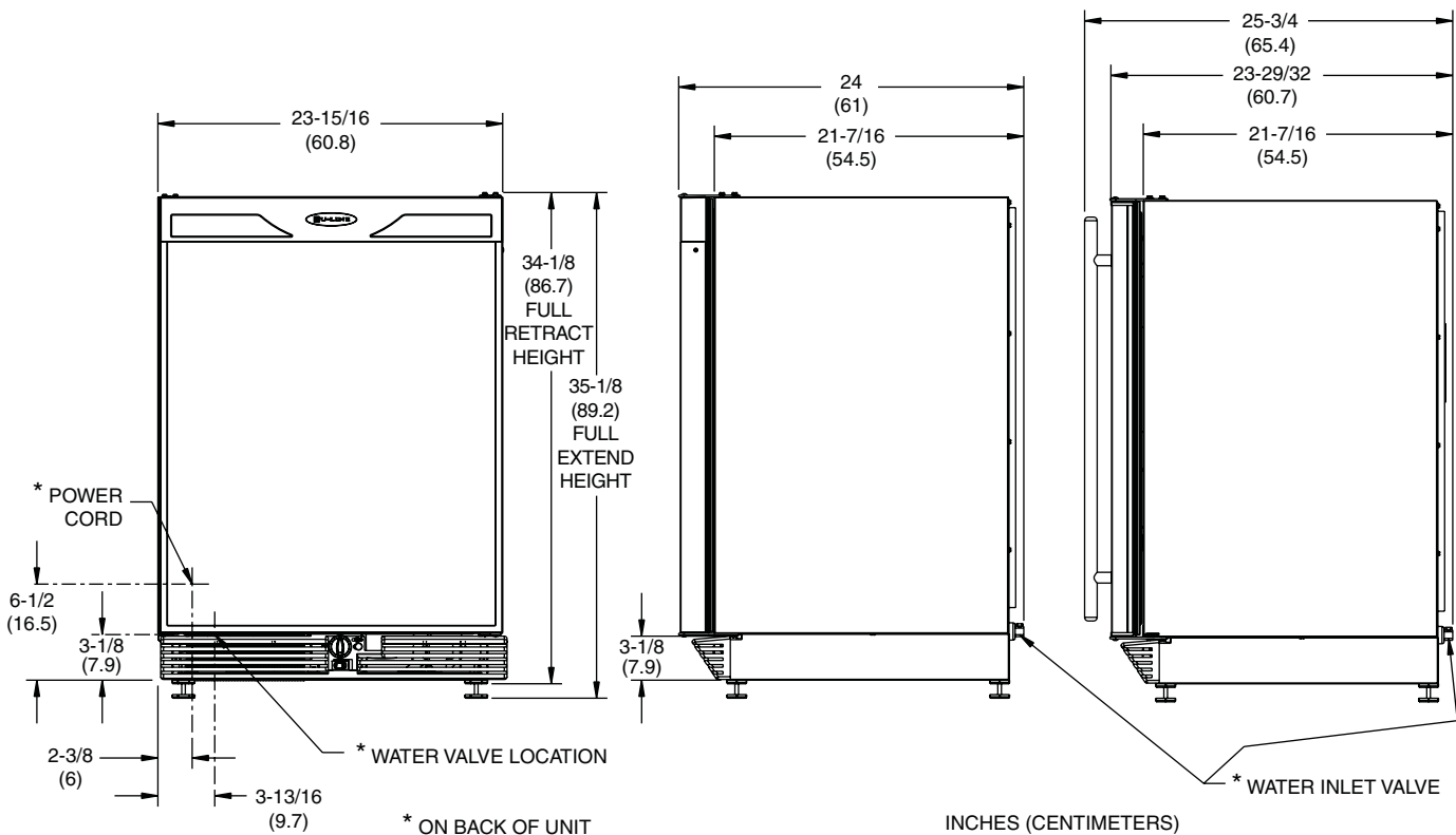
CO1175 (Stainless Steel)
