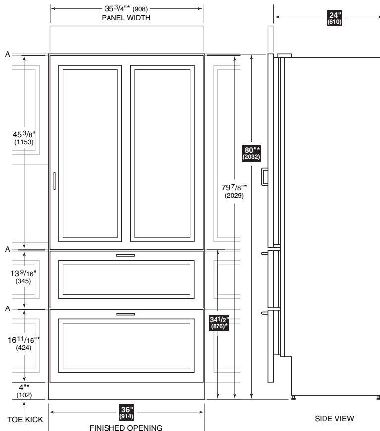
A) ALL REVEALS ARE 1/8" (3)
