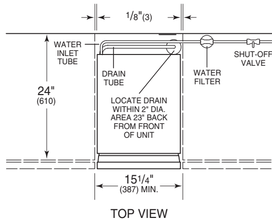
Model 315I - Gravity Drain
