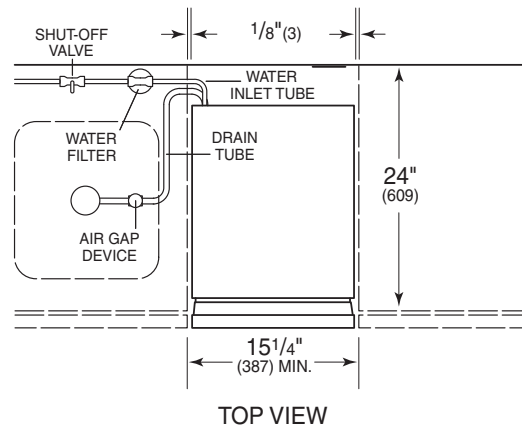
Model 315IP - Drain Pump
