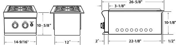
BGB132-BI Double Side Burner
