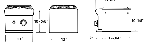
BGB132 Double Side Burner
