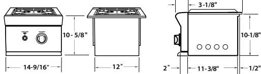
BGB132-BI Double Side Burner
