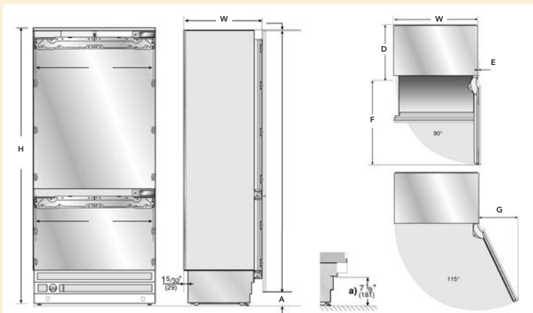
Integra Freezer B36IB70SSS – Stainless Steel B36IB70NSP – Custom Panel
