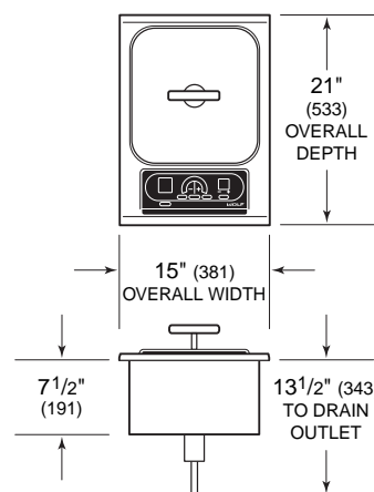
Electric Fryer Module
