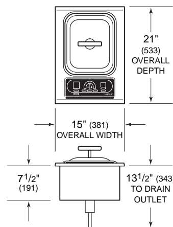
Electric Steamer Module
