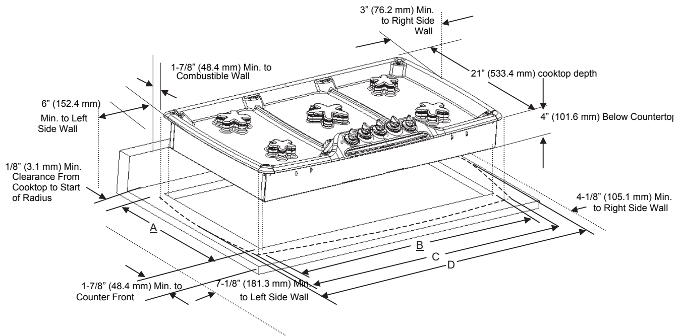
Figure 2: Cutout Dimensions
