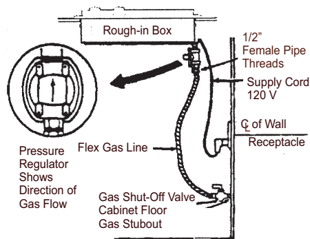
Figure 6: Gas and Electrical Location
