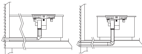
Thru Cabinet Toe Space
